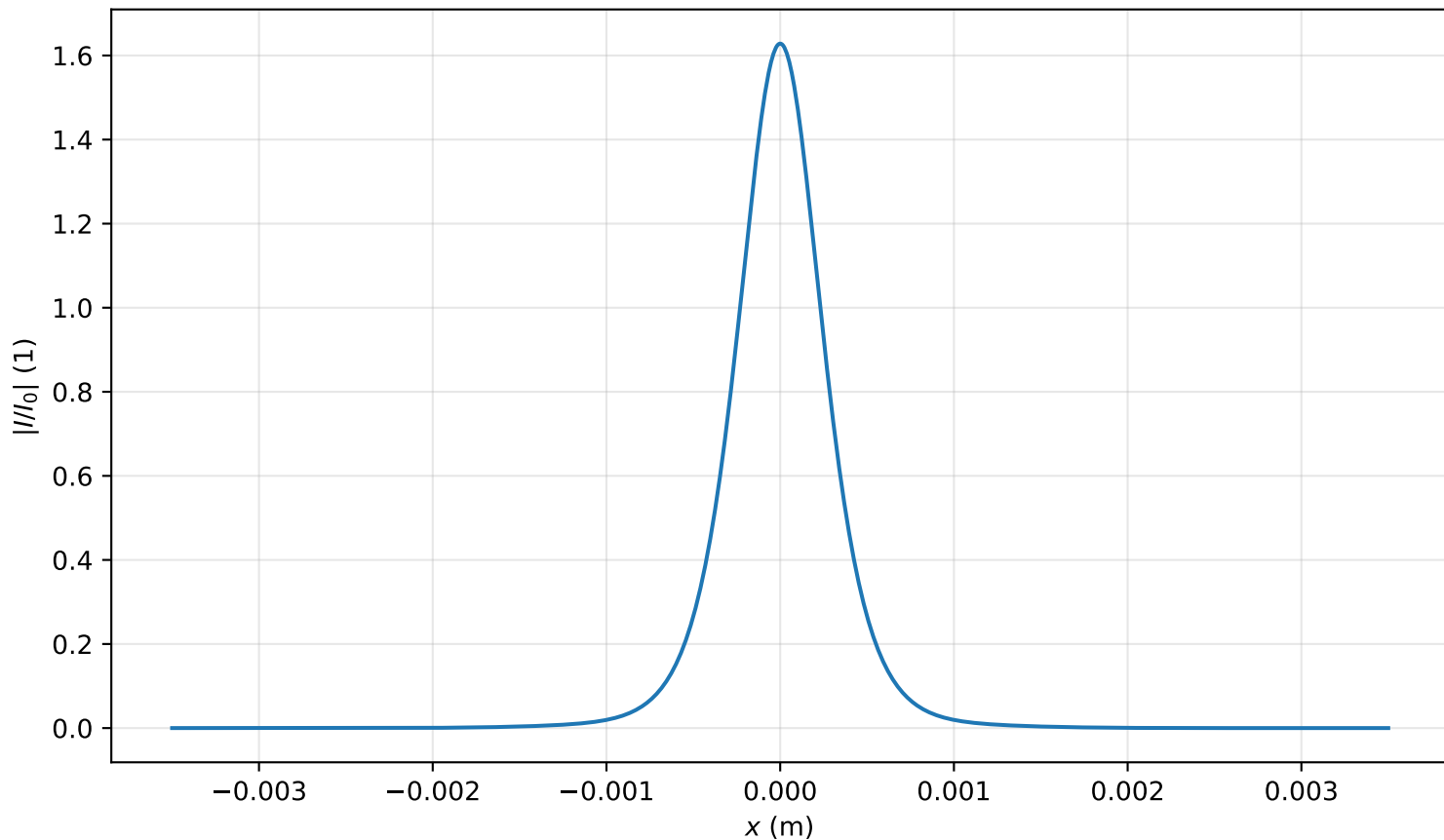
Intensity profile I(x, y = 0, z = 2.388m)/I_0 , P_{in}=0.9P_{cr} , artificial time
